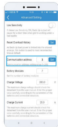
Figure 7. Configuration Page of PV Master
