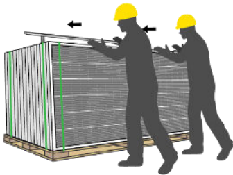
4) Cut off all the horizontal packing belts; when there are 1 or 2 vertical packing belts remaining, push the module gently to tilt toward the stand supporter.
