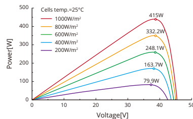
Power-Voltage Curve
