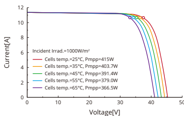
Current-Voltage Curve
